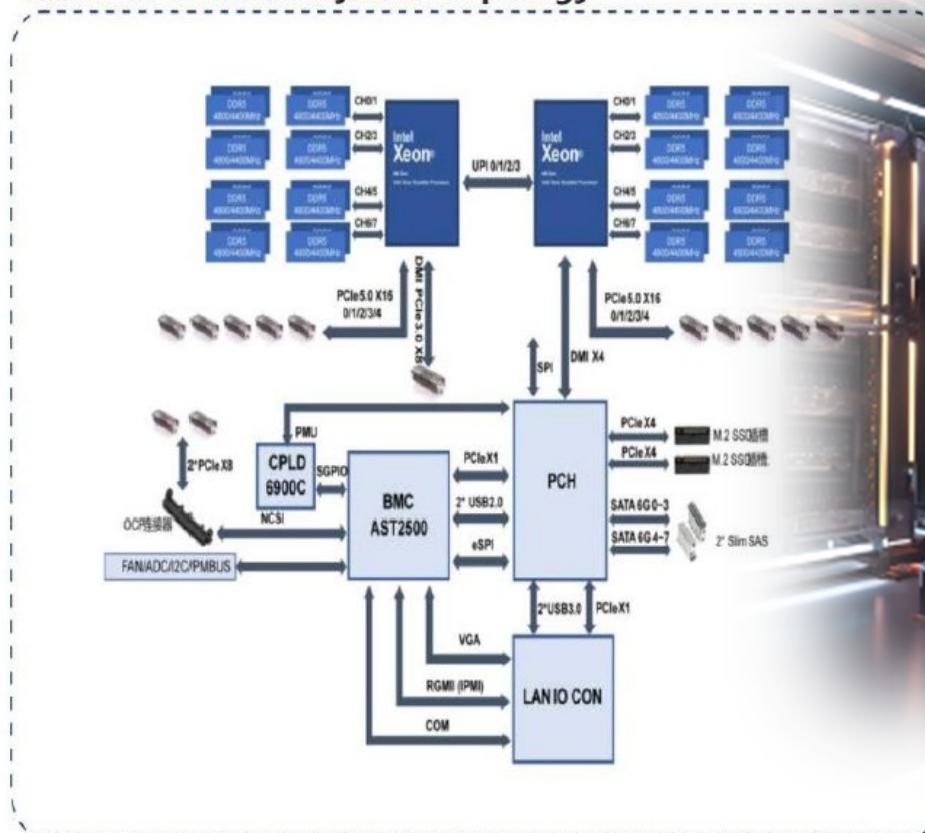
LINKWING H100 GPU Server System Topology
